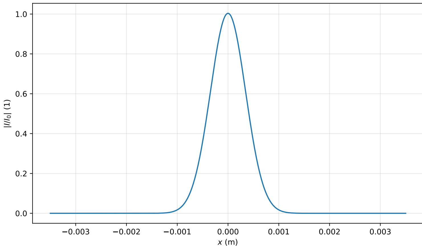
Intensity profile I(x, y = 0, z = 0.159m)/I_0 , P_{in}=0.4P_{cr} , artificial time
